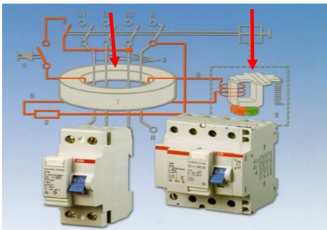
Fig. 9. Basic GFCI design (European version)
