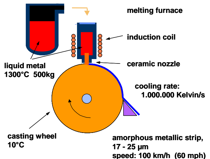
Fig. 3. Rapid Solidification Technology
