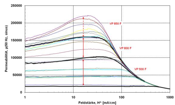
Fig. 4b. Grades of B(H) shapes, from very linear (and flat) to almost round. Standard series cores go up to about \mu ca. 100.000
