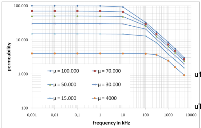
Fig. 5. Permeability versus frequency of nanocrystalline cores with different permeability levels
