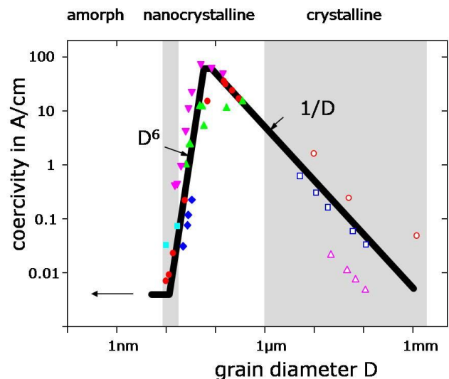
Fig. 2. The famous D^6 law from Dr. Herzer: making things smaller will sometimes surprise you
