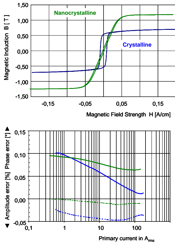
Fig. 8. Basic differences between crystalline and nanocrystalline high-permeability alloys for precise current transformers
