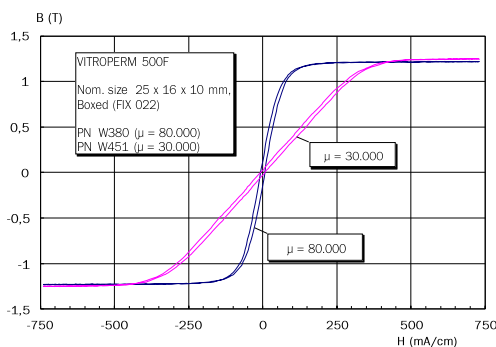
Fig. 4a. Static hysteresis loops and permeability versus field strength of nanocrystalline standard cores with different permeability levels.
